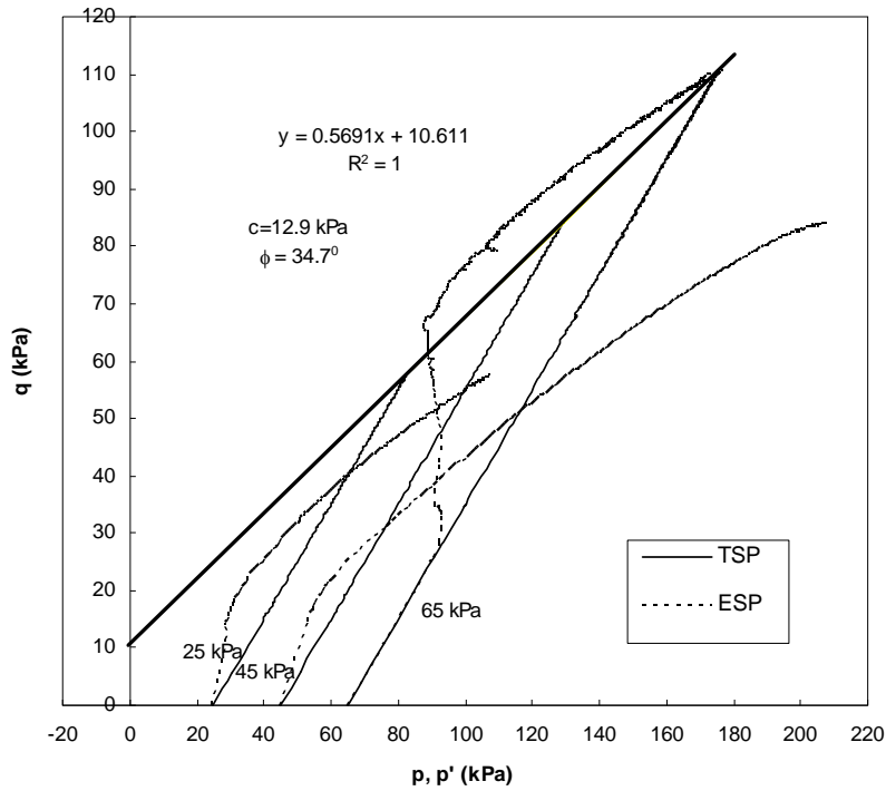
Figure 5.11: Stress path for BH1
